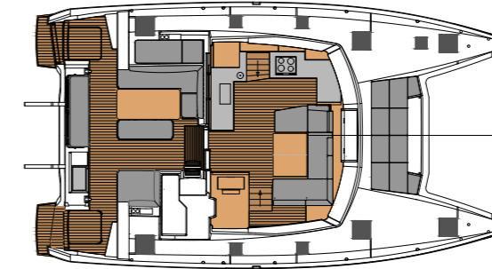
SALOON
