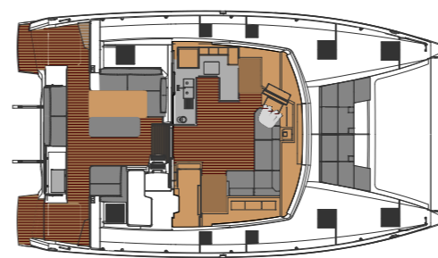
DECK
